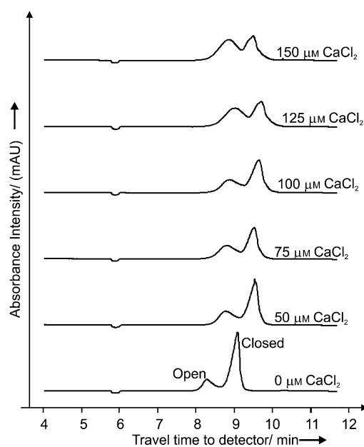
Figure 3. KCE of TG2 showing the influence of increasing concentrations (50 to 150 \mu\text{M} ) of calcium chloride on the equilibrium distribution of the open and closed conformations.
